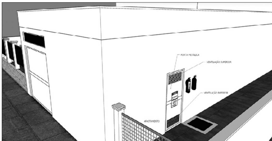
Figura 04: Central de GLP – “nicho”
